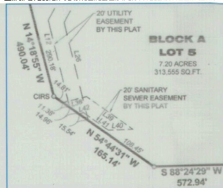
DETAIL "A" (1" = 80')
